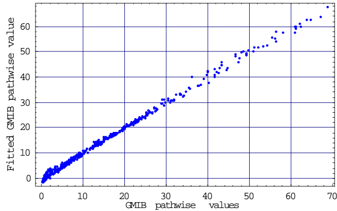
Figure 2. Scattered plot of fitted GMIB pathwise values against GMIB pathwise values
