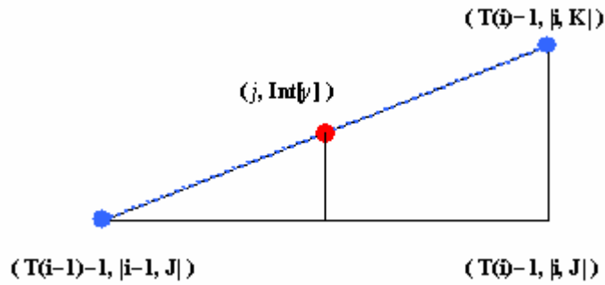
Figure 5. Branch b(i, J, K)
