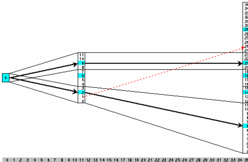
Figure 6. Representative Paths and Their Probabilities
