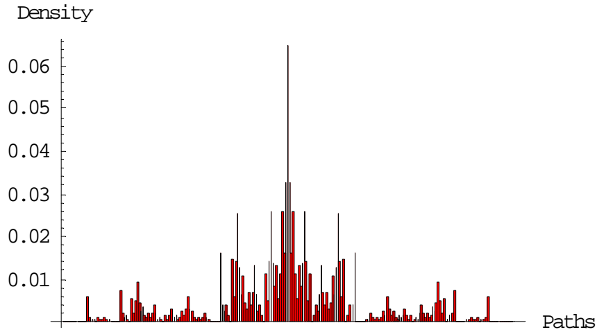
Figure 7. Representative Path Probability of LPS Model
